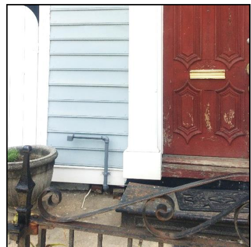
For existing structures, meter may be placed on front façade if it is a safety risk to be located elsewhere. A pressure relief vent may be located on the front or side façade. Paint all to match adjacent wall color.
